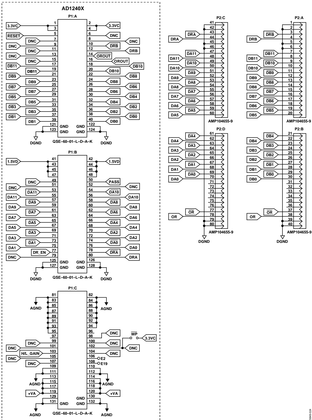
Figure 25. Evaluation Board
